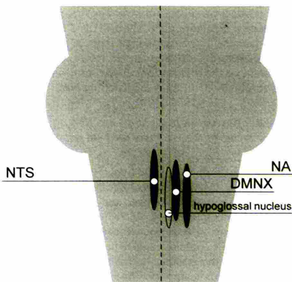
Figure 1. Primary brainstem nuclei of the vagus. Nuclei are bilateral, and only one of each bilateral pair is illustrated.
